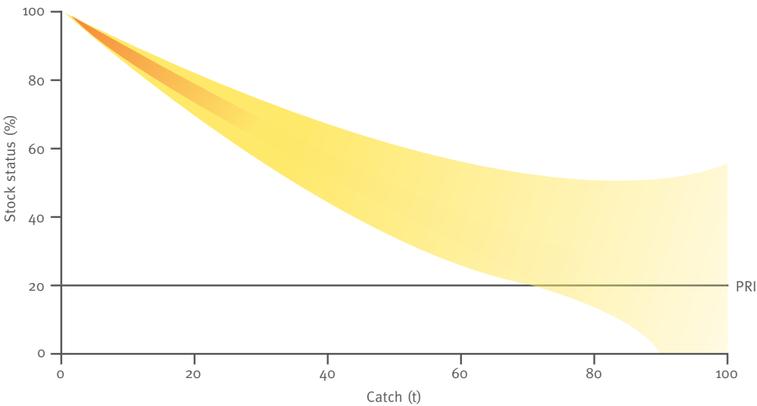
Figure 1 – This diagram illustrates how uncertainty increases with the level of exploitation (catch). In a watercolour plot, probability is represented by the density of ink, so as the values become increasing uncertain, the ink washes out over a greater range of values. In this diagram, when catches are zero or very small, we are certain the stock is close to unexploited (100% stock status). As catches increase, not only do we see that the stock status decreases further below the unexploited level, but the actual status becomes increasingly uncertain. The critical issue is, for any exploitation level (catch), how much probability (ink density) is below the PRI (solid horizontal line).
