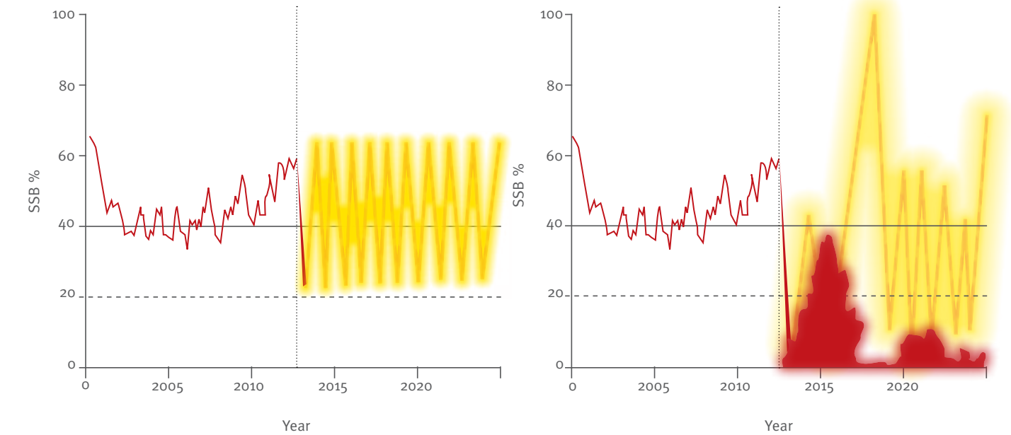
Figure 4 – The graphs illustrate how stock assessment projections might be used to test harvest control rules and provide evidence that a particular HCR is sustainable. The graphs show a stock assessment for a shrimp species for two harvest control rules. In both cases, the stock assessment indicates the stock status to 2013, to the left of the vertical dotted line. To the right of the line, different HCR have been applied. Uncertainty is represented by ink density, and red histograms in the right-hand graph indicate stock collapse. The simulation clearly indicates the HCR tested on the right is not precautionary.
