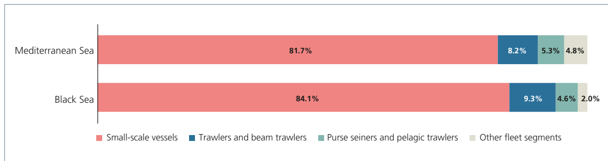
FIGURE 8. Fleet segment composition in the Mediterranean and the Black Sea
