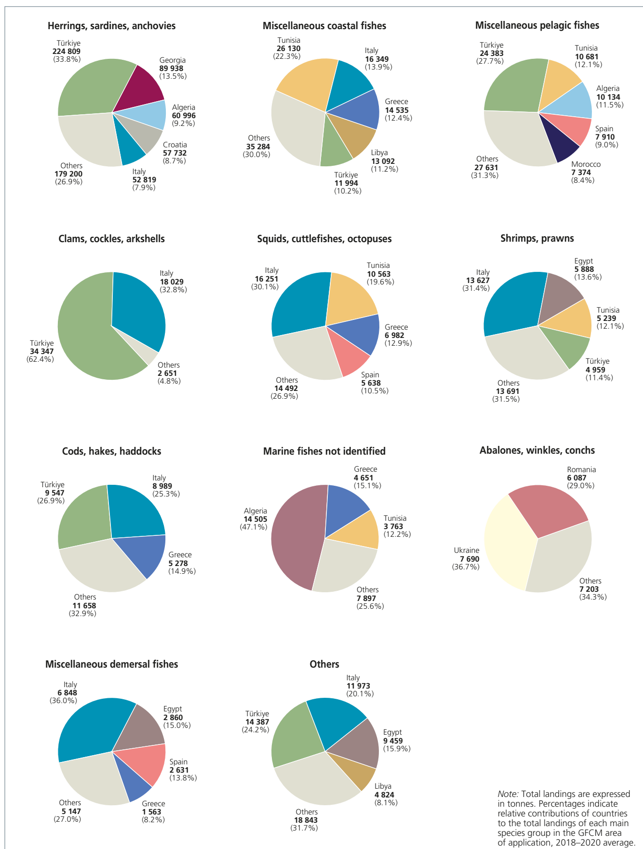
FIGURE 20. Total landings of main species groups by country in the GFCM area of application, 2018–2020 average
