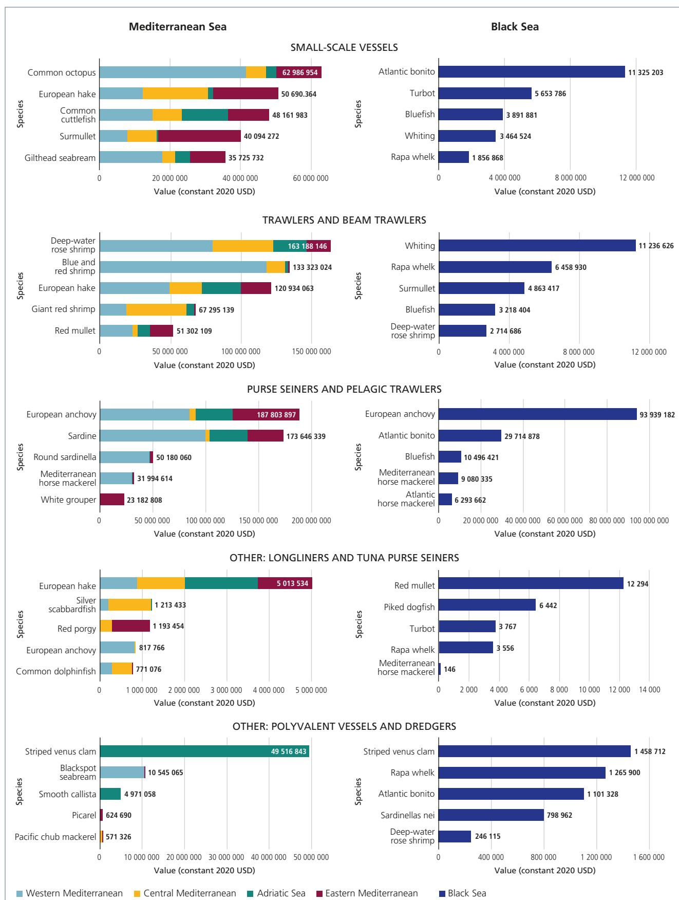
FIGURE 41. Top five commercial species (in terms of value) by fleet segment group in the Mediterranean subregions and in the Black Sea
