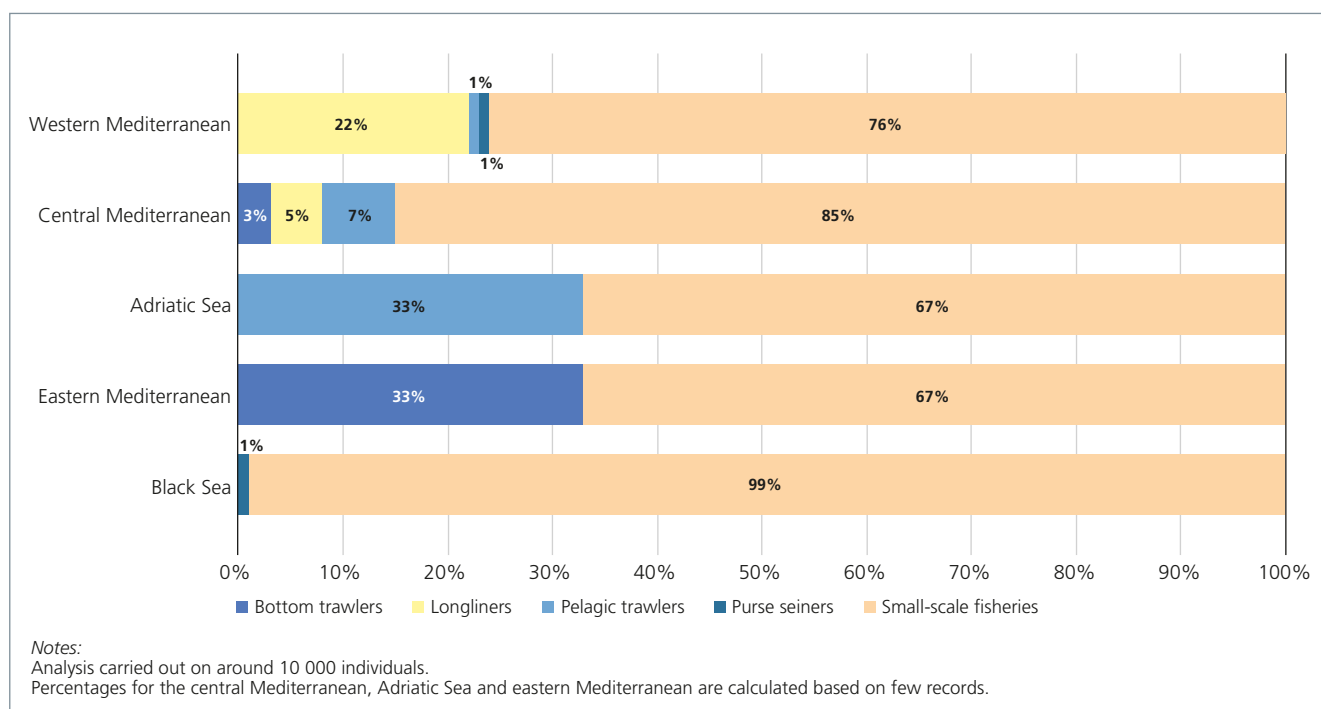
FIGURE 69. Relative contributions of main vessel groups to the total incidental catch of cetaceans by GFCM subregion, 2000–2022
