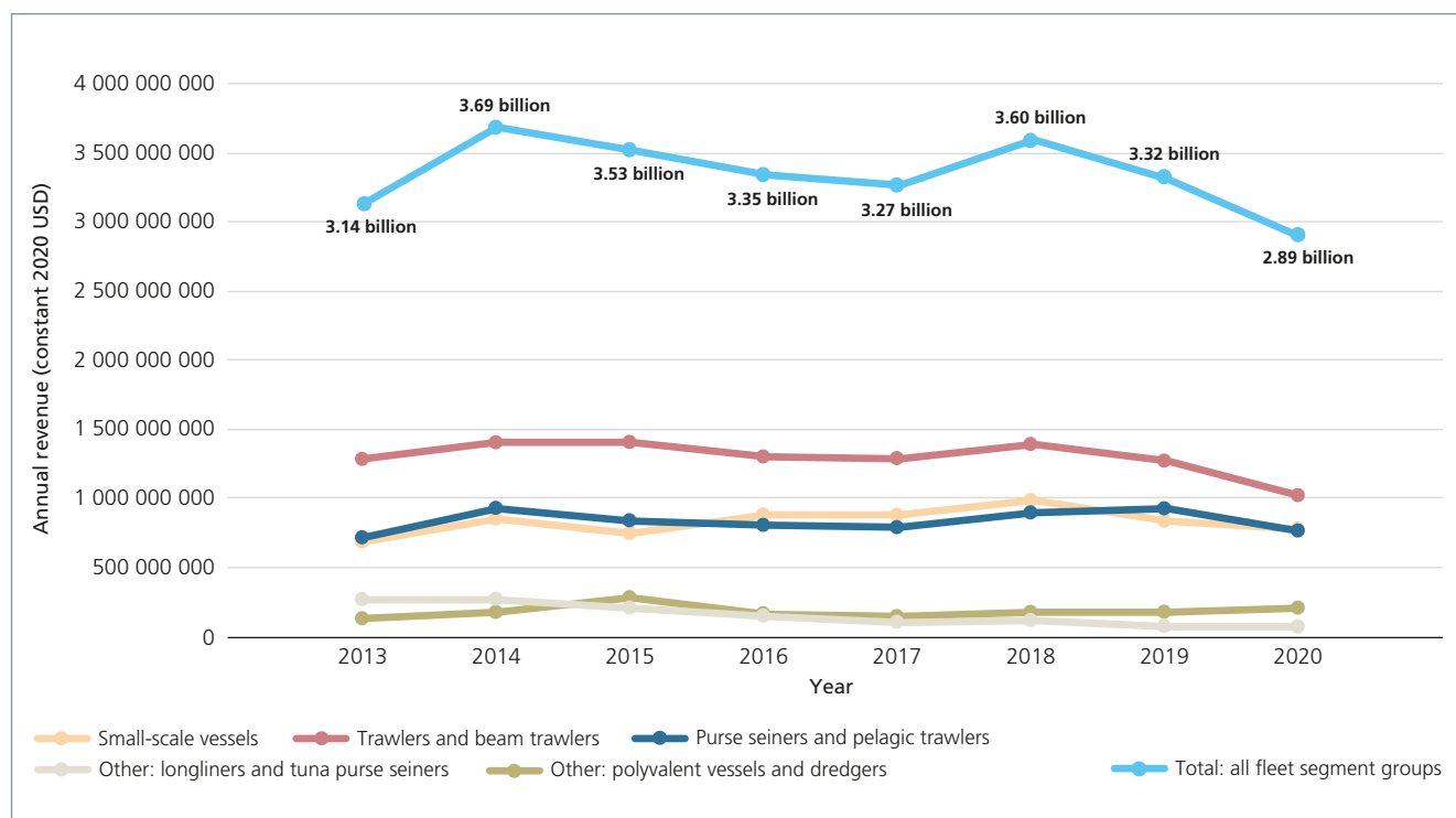
FIGURE 34. Revenue from marine capture fisheries per year by fleet segment group in the GFCM area of application, 2013–2020
