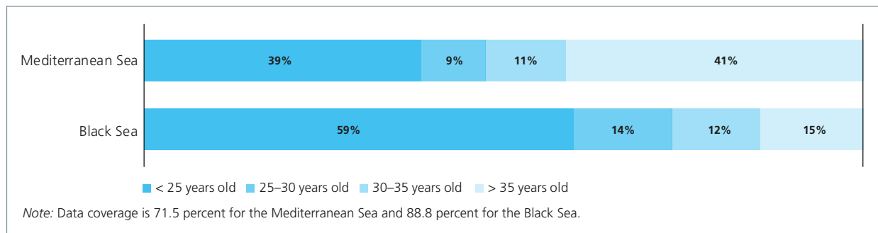
FIGURE 5. Age composition of the fishing fleet in the Mediterranean and the Black Sea
