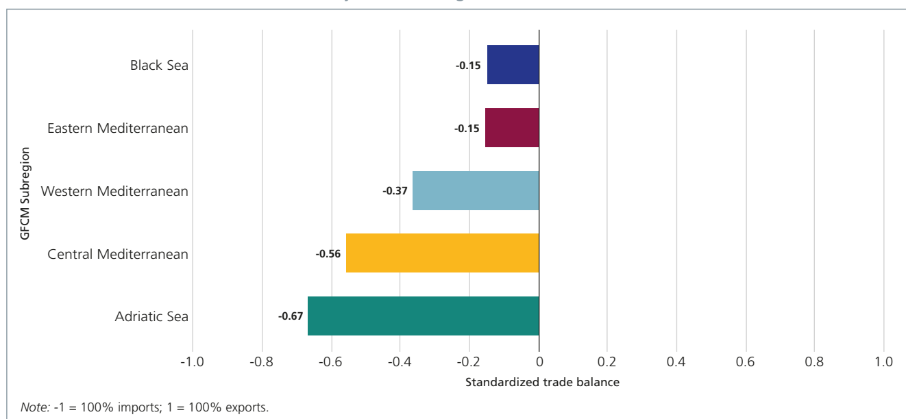
FIGURE 56. Standardized trade balance by GFCM subregion
