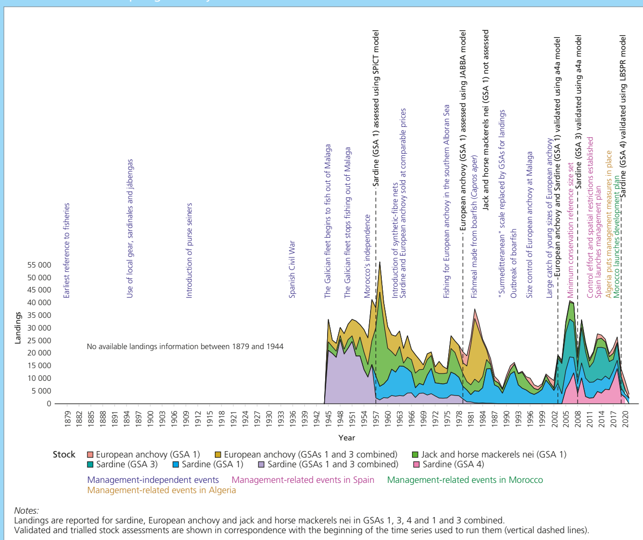
Timeline of the small pelagic fishery in the Alboran Sea
