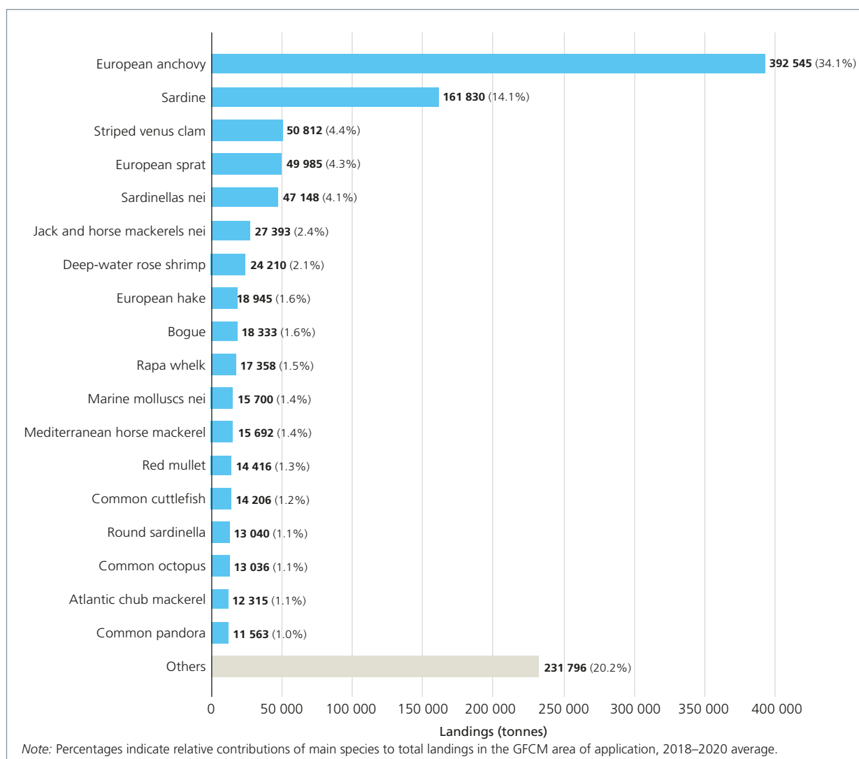
FIGURE 23. Total landings by main species contributing at least 1 percent of the total catch in the GFCM area of application, 2018–2020 average
