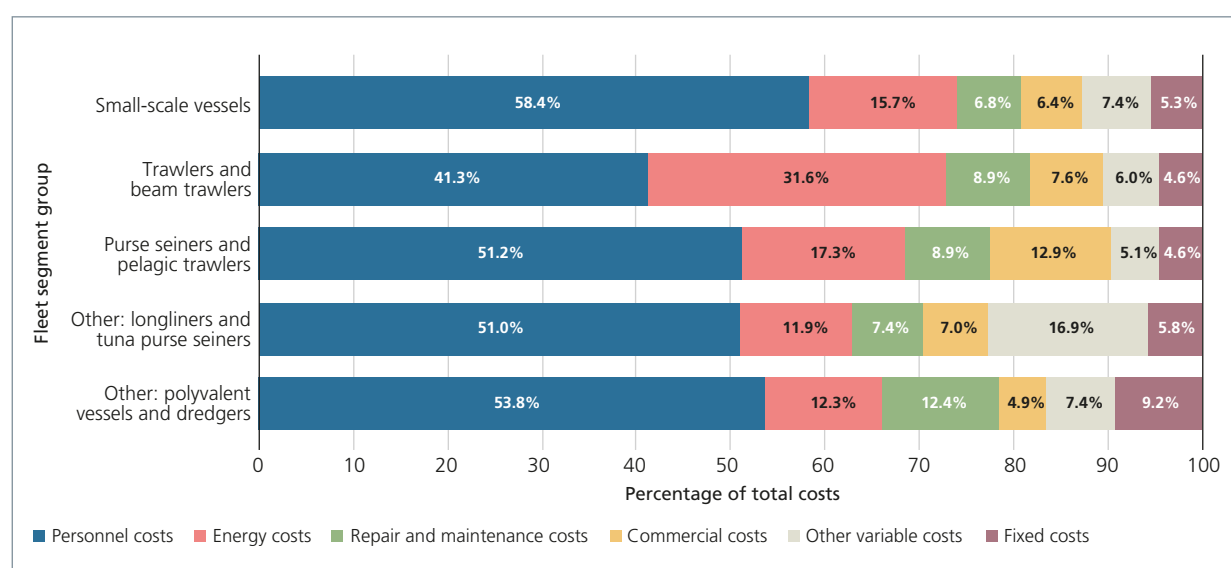
FIGURE 44. Operating cost structure (as a percentage of the total costs) by fleet segment group
