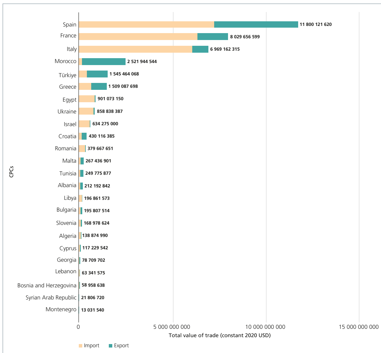
FIGURE 54. Total value of traded fish products by GFCM contracting party and cooperating non-contracting party (imports and exports)
