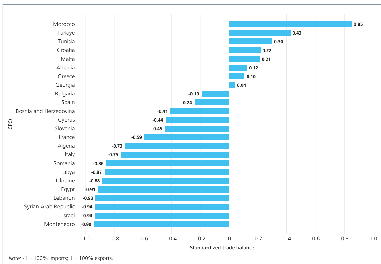
FIGURE 55. Standardized trade balance by GFCM contracting party and cooperating non-contracting party
