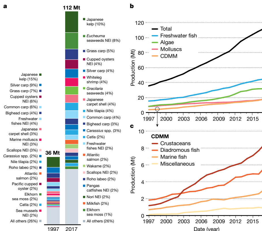
Fig. 1 | Composition and growth of global live-weight aquaculture production. a, The species composition is shown for 1997 and 2017. Green, plants and algae; blue, freshwater fish; pink, shellfish; orange, diadromous fish. b, c, Growth is shown from 1997 to 2017 for the following production categories ( b ): total, freshwater fish, algae, molluscs and CDDM, which comprises crustaceans, diadromous fish, marine fish, and miscellaneous species and is
