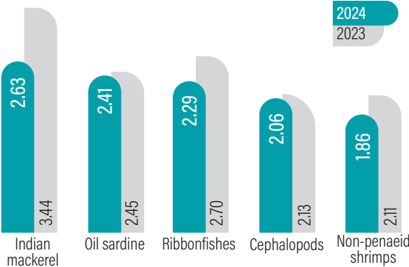
Major species/groups with their contribution (lakh tonnes) towards total marine fish landings in India
