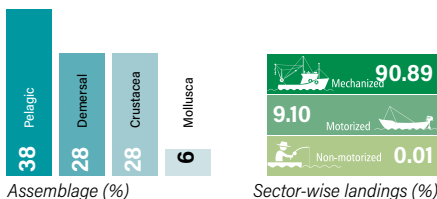
Assemblage (%)
