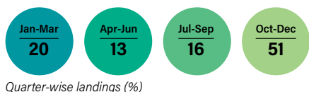
Quarter-wise landings (%)
