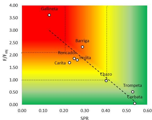
Reproductive Potential Ratio (SPR) vs Relative Fishing Mortality ( F / F_{obj} ) for the 8 main benthopelagic species caught in the small pelagic fishery of Ecuador.
