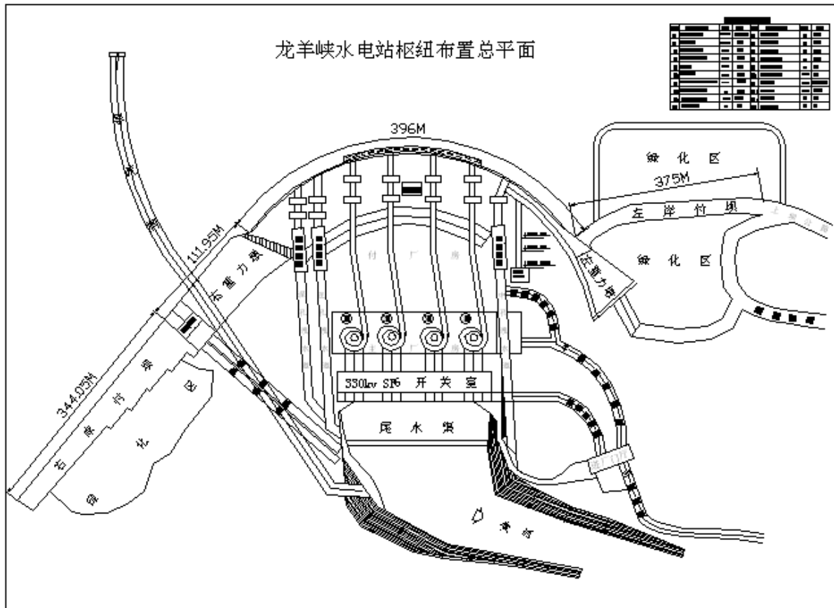
General layout of Longyangxia Hydropower Project
