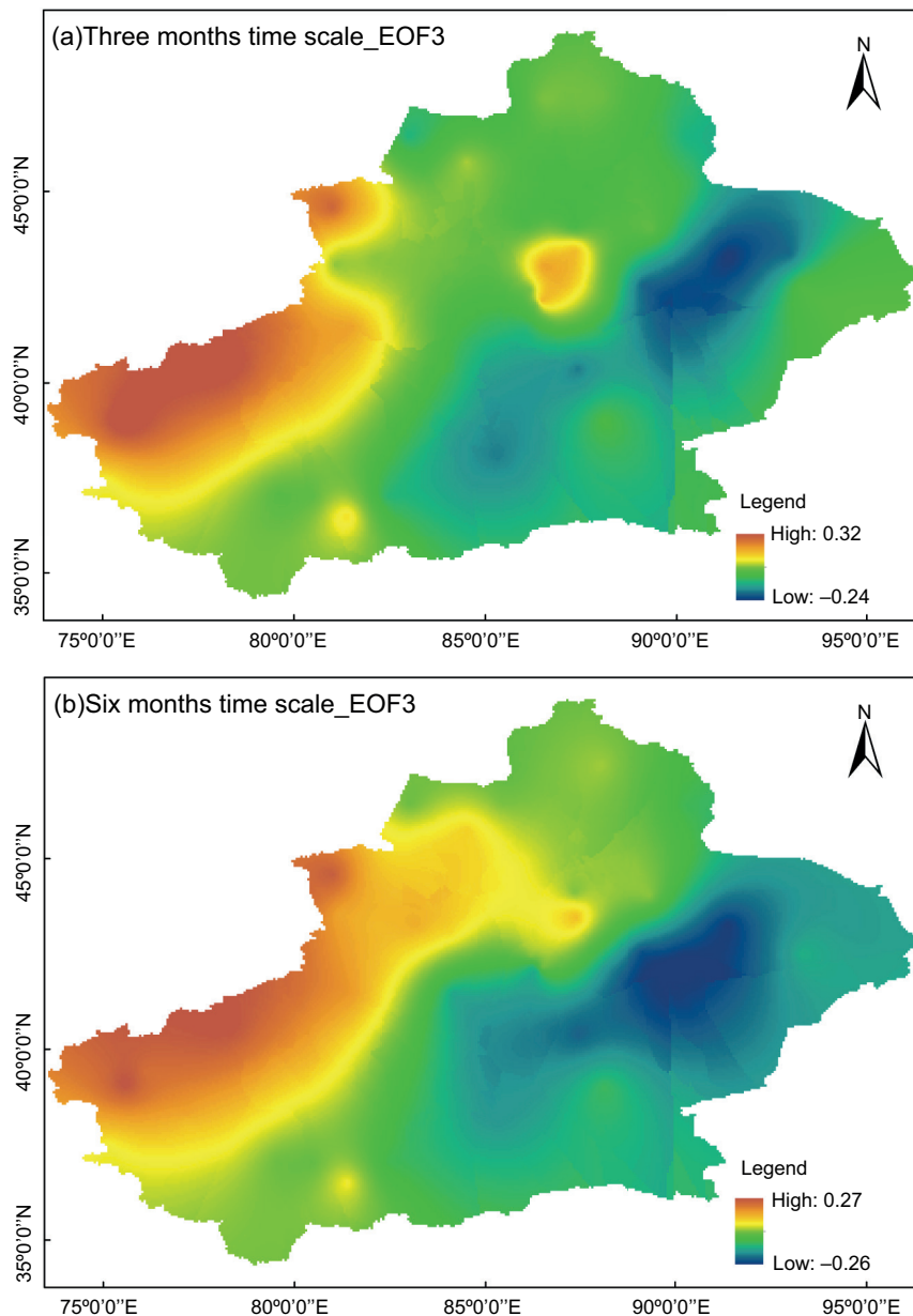
Fig. 7. Spatial distribution of the third mode of the (a) three-month time scale and (b) the six-month time scale in Xinjiang.
